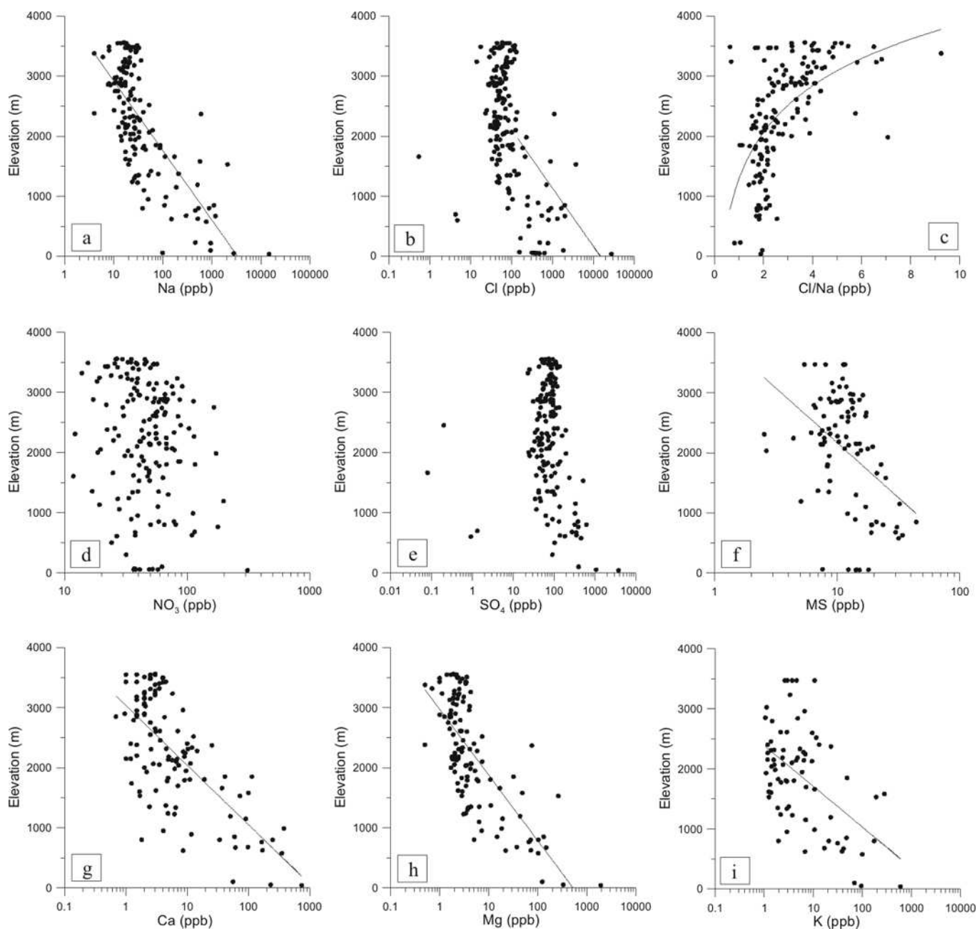
Fig. 2. Relationship between multi-year ion concentration data and elevation: (a) Na; (b) Cl; (c) Cl/Na ratio; (d) NO 3 ; (e) SO 4 ; (f) MS; (g) Ca; (h) Mg; and (i) K. All species are plotted on a logarithmic scale, except for (c) which is plotted on a linear scale. The logarithmic trends shown are significant on the 99.9% level.
