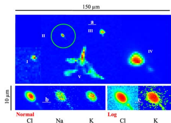
Figure 4. Brine inclusions at 3551 m. Probe size: from 0.3 \times 0.5 \mu\text{m} (II and III) to 1 \times 1 \mu\text{m} (I, IV and V); exciting energy: 4.5 keV. See Figure 3 for concentration scaling.
