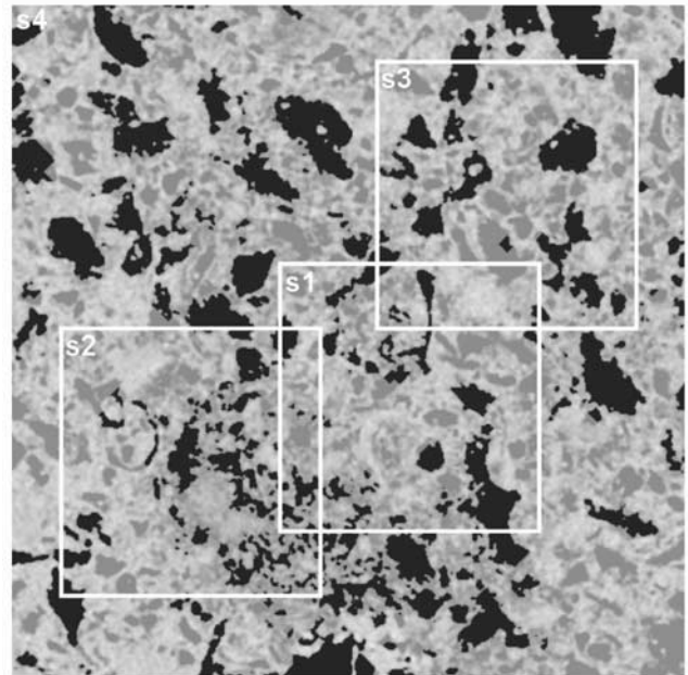
Figure 4. Locations of cross sections S1, S2, and S3 (size 1 mm \times 1 mm) in the cross section S4 (size 2.5 mm \times 2.5 mm).
