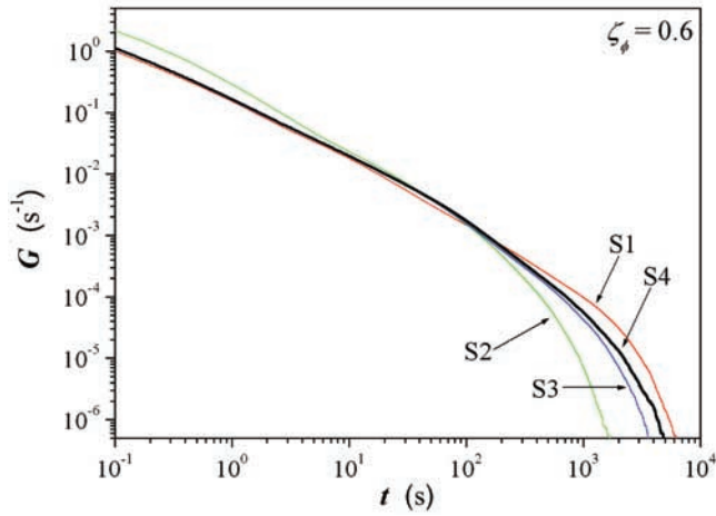
Figure 15. Memory function computed for subdomains S1, S2, S3 ( 200 \times 200 pixels), and S4 ( 510 \times 510 pixels), located as indicated in Figure 4.
