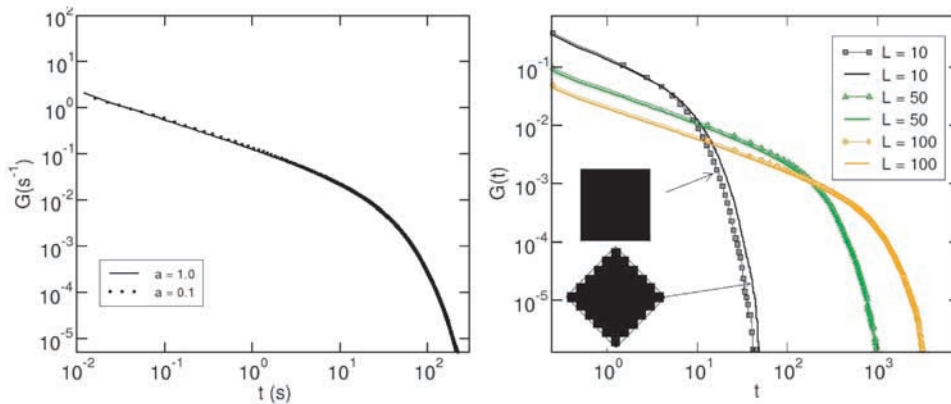
Figure 12. (left) Memory function G(t) computed for cross section S1 for a = 1 and 0.1. (right) G(t) computed for square-shaped immobile domains of length L = 10 , 50, and 100 pixels ( \phi_m = 1 ). By rotating the square, the mobile-immobile surface, S_{\Omega} , and the mobile-immobile interface roughness are artificially increased. As L increases, the ratio S_{\Omega}/V_{im} for the rotated square tends to equal that of the nonrotated square, and the difference between the memory function computed for the rotated and the nonrotated square tends to cancel. However, these results show that the main effect introduced by the artificial increase of S_{\Omega}/V_{im} is, as expected, on the memory function breakthrough time and not on the early time slope.
