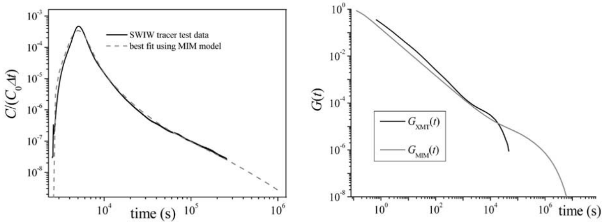
Figure 13. (left) Best fit of the SWIW tracer test BTC for a tracer flush duration of 2400 s using TRANSIN solver. (right) Corresponding memory ( G_{MIM} ) compared to the memory function G_{XMT} computed using the XMT cross section S4.
