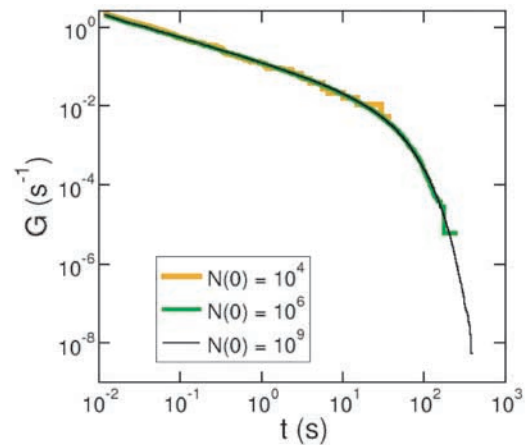
Figure 10. Computed memory function corresponding to the cross sections displayed in Figure 11 for an increasing number of random walkers N(0) ( N(0) = 10^4, 10^6 , and 10^9 , respectively).
