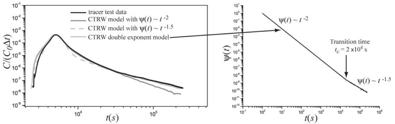
Figure 1. (left) Example of breakthrough curve (BTC) obtained from SWIW tracing experiment at depth 94 m in well MC2 (Ses Sitjoles test site) and CTRW model fitted curves. Concentration, C , is normalized by dividing it by C_0 , the concentration of the injected tracer, and the injection duration, \Delta t . The unusual shape of the curve tail is modeled by a MIM mass transfer model using the CTRW approach with a dual-slope transition time distribution [Le Borgne and Gouze, 2008]. (right) Dual slope transition time distribution used in the CTRW computations to account for the retention time probability of the tracer in the immobile domain.
