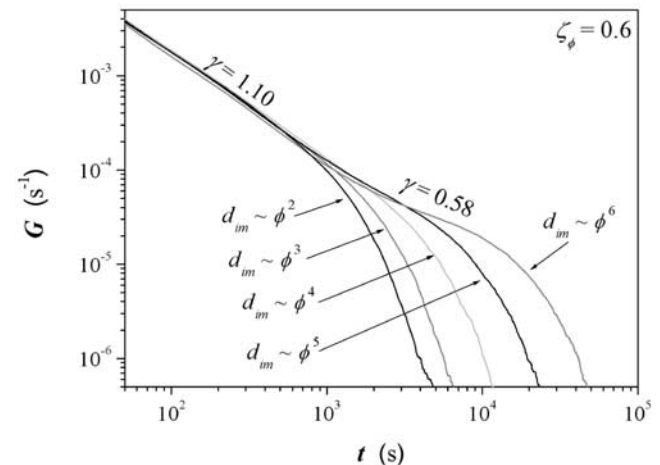
Figure 16. Memory function computed for increasing values of n ( 1 < n < 5 ) with d_{im} \sim (\phi'_{im})^{n+1} .
