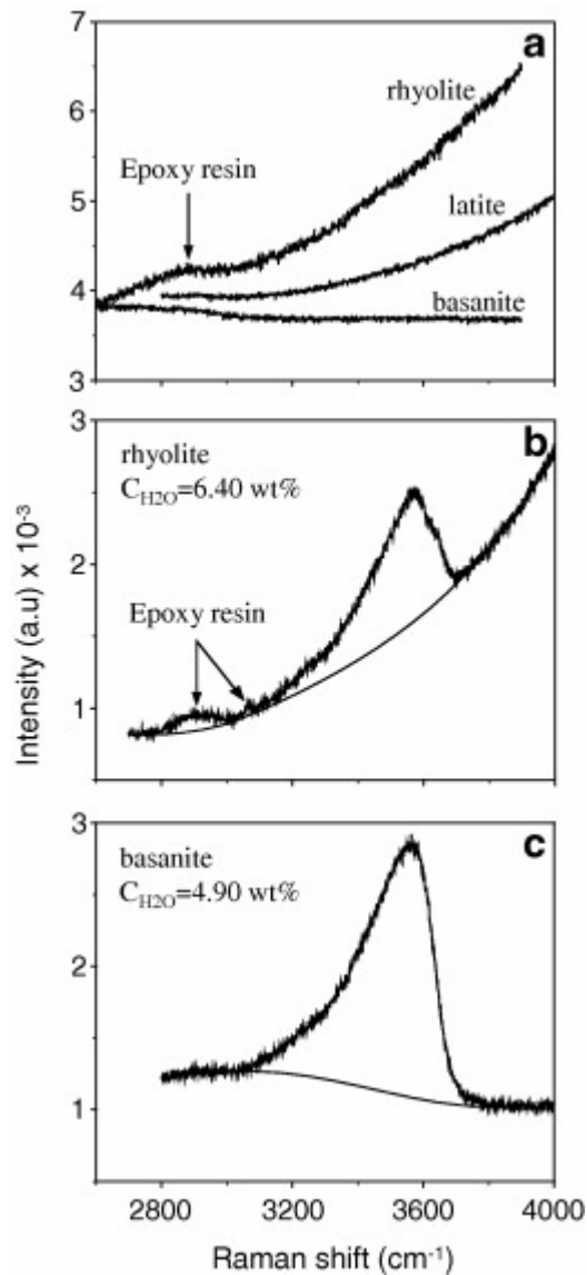
Fig. 3. (a) Raman spectra of dry glass samples with decreasing transparency from rhyolite to basanite. Fluorescence backgrounds are produced by the excitation of embedding resin and are best fitted by a cubic baseline. Comparison between uncorrected Raman spectra with the appropriate baseline correction for (b) a metaluminous rhyolite glass with 6.40 wt% of water content and (c) a basanitic Sommata glass with 4.90 wt% of water content demonstrates that a linear baseline approximate the background only in dark mafic glasses. All the absolute intensities have been divided by 1000.
