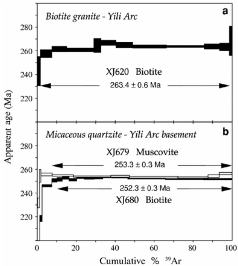
Fig. 4 ^{40}\text{Ar}/^{39}\text{Ar} age spectra acquired by laser step heating of a biotite single grain XJ620 from a Carboniferous biotite granite of the Yili arc (a) and muscovite XJ679 and biotite XJ680 (b) single grains from micaceous quartzites from the metamorphosed and ductilely deformed sedimentary cover of the crystalline basement of the southern margin of the Yili arc
