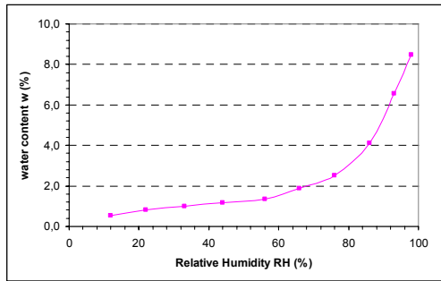
Fig. 7. Water retention curve of tuffeau
