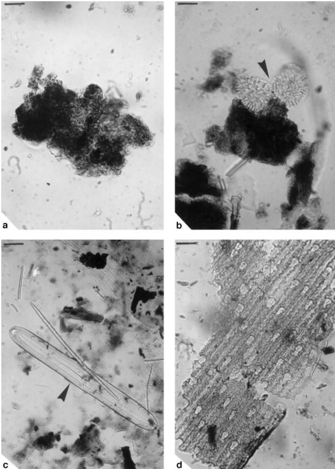
Plate. 1. Micrographs of peat samples from Trittivakely marsh, Madagascar, obtained by transmitted light microscopy. (a): Amorphous organic matter flakes derived from destructureation and alteration of higher plant tissues and occurring in large amount throughout the peat profile. (b) and (c): Algal organic matter composed of Botryococcus (b) (arrow) and diatoms (c) (arrow) which occurs as a minor fraction in the half upper part of the peat profile. (d): Well-preserved plant tissues of Cyperaceae occurring in substantial proportions in the surface peat ( \leq 10 cm depth). Scale bar=15 \mu m.
