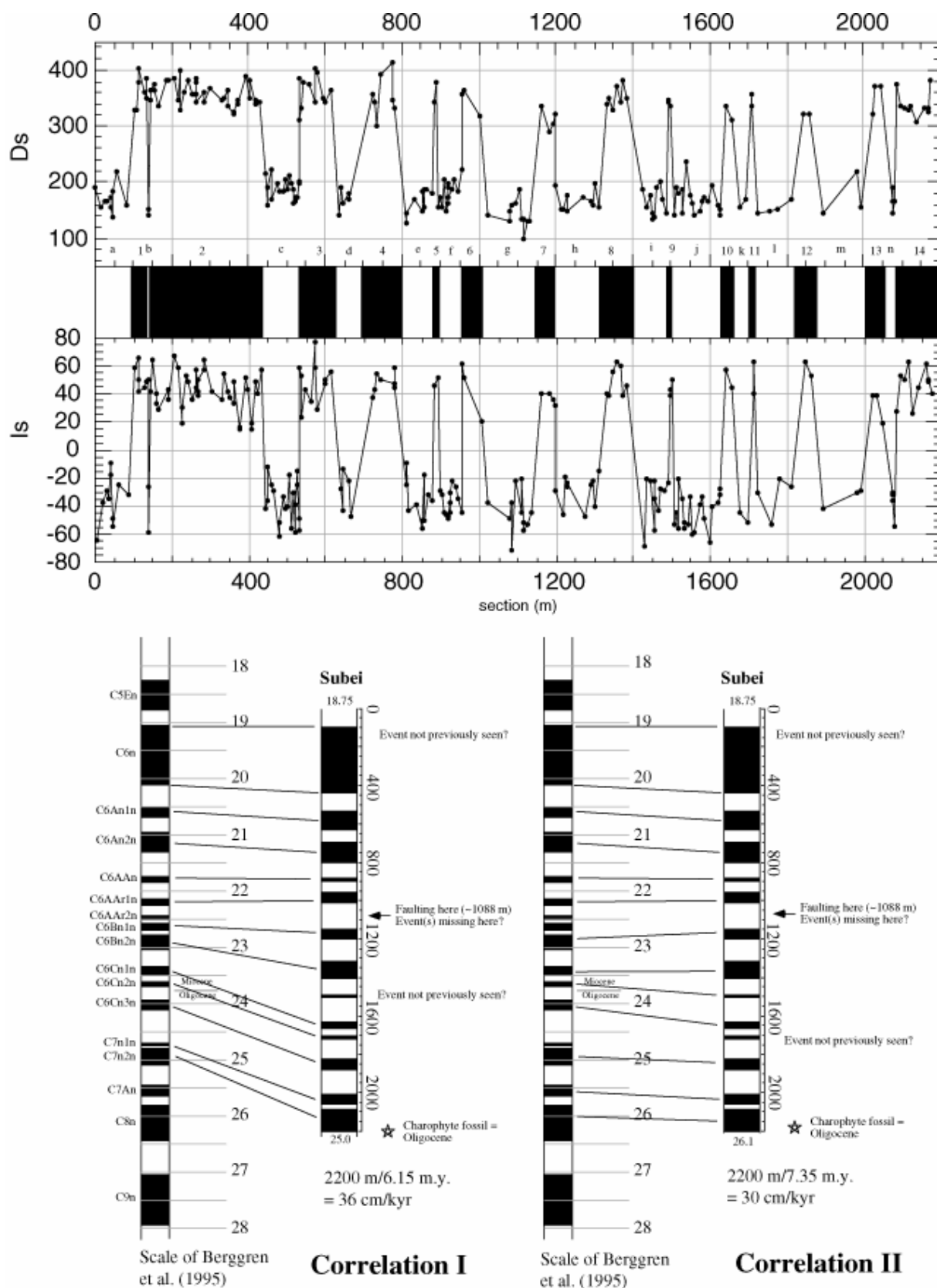
Figure 5. (top) Magnetic polarity scale of the Xishuigou section, Subei, and (bottom) two correlations with the reference scale of Berggren et al. [1995]. Normal polarity reference chronos are listed on left scale.
