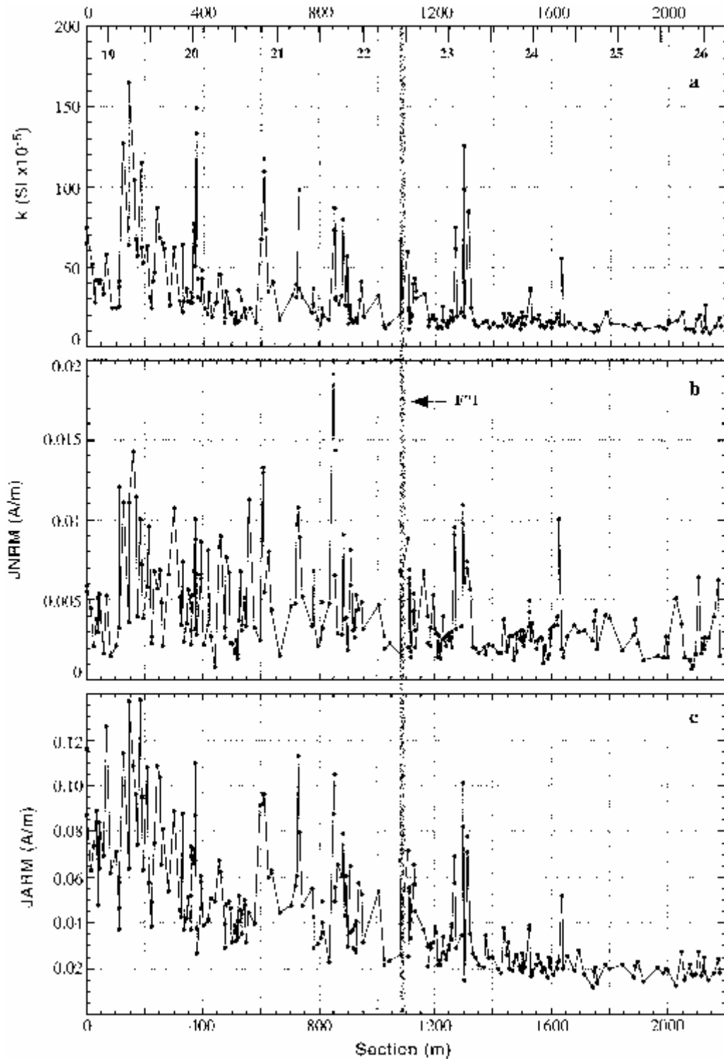
Figure 8. (a) Bulk susceptibility ( k ), (b) NRM intensity ( JNRM ), and (c) anhysteretic remanent magnetization intensity ( JARM ) plotted against depth (0 is top; 2179 m is bottom). Scale in Ma from correlation II of Figure 5 is provided in Figure 8a.
