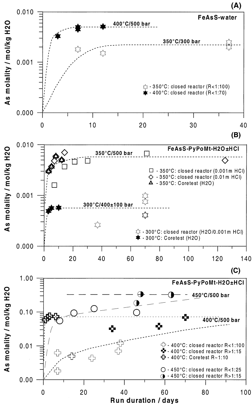
Fig. 2. Arsenic concentrations measured as a function of time in arsenopyrite dissolution runs conducted in pure water without buffer (A), in H 2 O-HCl solutions in the presence of PyPoMt assemblage at 300 and 350°C (B), and at 400 and 450°C (C). The symbols denote different runs at indicated conditions (see text and Tables 1 and 2 for details). The dashed lines are drawn to aid the eye. It can be seen that similar steady states for As concentration are attained at the same T-P conditions for experiments carried out either by quenching (closed reactor) or sampling (Coretest) and with different solid/solution ratios and acidities (~HCl concentration).
