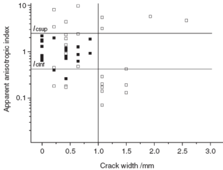
Figure 6 Variation of the apparent anisotropic index with respect to average crack width within each unit area: & cracks that do not cross and & cracks that cross the in-line MN ( l_{cinf} and l_{csup} are the two thresholds determined for crack identification >1 mm).
