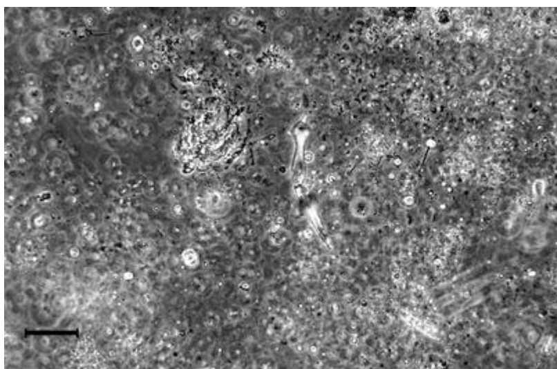
Fig. 3 Heterogeneous structure of surface macroaggregates. Among a variety of organisms and particles, some amoeboid structures can be observed ( scale bar 60 μm)
