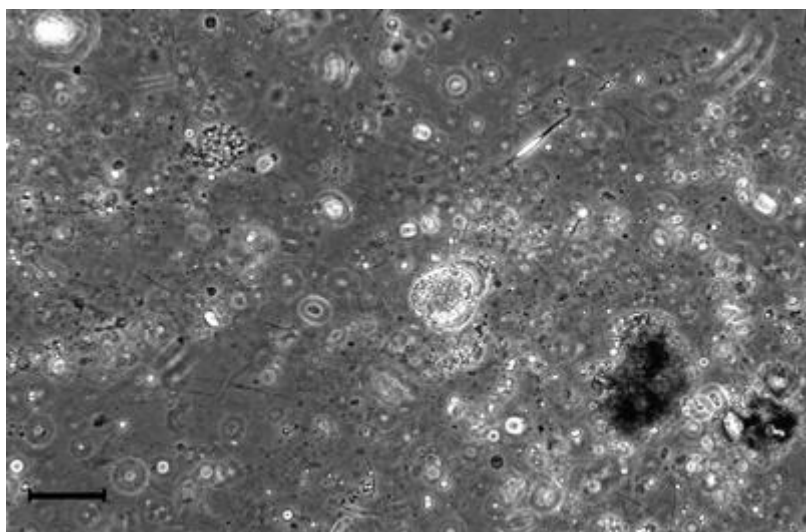
Fig. 4 Surface macroaggregates. Some naked Gymnodinium -like dinoflagellate can be observed (scale bar 60 \mu\text{m} )
